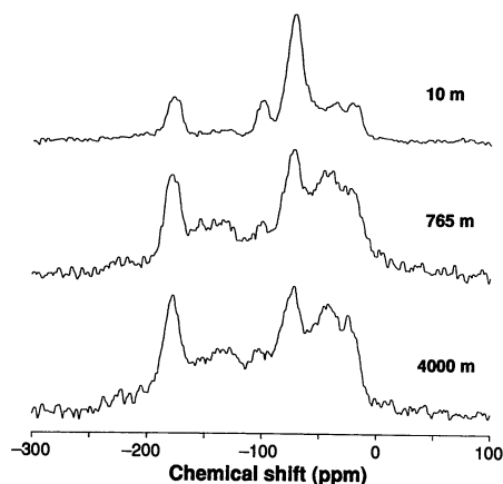
Fig. 1. Conventional CP/MAS ^{13}\text{C} NMR spectra of DOM isolated by ultrafiltration (>1000 daltons) from surface water (10 m), oxygen-minimum water (765 m), and deep water (4000 m) at 22°45'N, 158°00'W in the Pacific Ocean.
